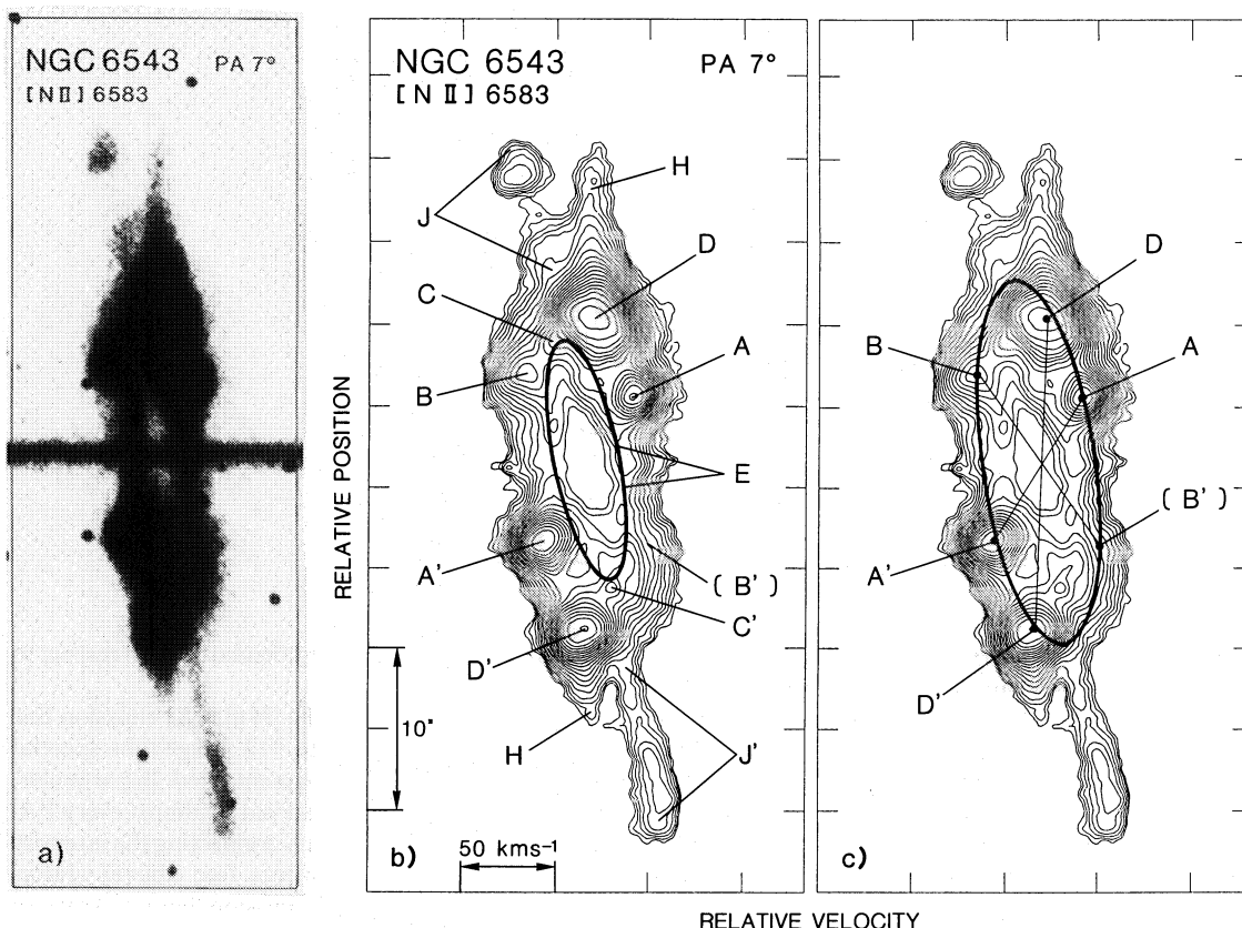
Fig. 3. a Enlarged high-resolution long-slit spectrogram of NGC6543 obtained at PA 7^\circ showing the [N II] 6583 line. The original dispersion is 1.8 \text{ \AA mm}^{-1} . b Position-velocity map of the line feature shown in the left-hand panel. The stellar continuum has been subtracted. The contour spacing is logarithmic, corresponding to a factor 2^{1/2} in intensity. The line feature is resolved into a large number of components which are arranged in a point symmetric pattern with respect to the center. For each component in the northern half of the line feature, a counterpart can be found in the southern half. Components in the northern half are denoted by A, B, C, D and J, their counterparts in the southern half by A', B', C', D' and J'. The central elliptical feature E (see text) is marked (continuous line). c Same as in the center panel. The intensity peaks of the two components of each pair are connected by a straight line. All lines virtually intersect in a single point which coincides with the centroid of the entire line feature. The centroid of the line feature coincides with the stellar position and represents the systemic radial velocity V_\odot = -63.5 \text{ km s}^{-1} . The intensity peaks of these components (except JJ') trace an outer ellipse, as indicated
