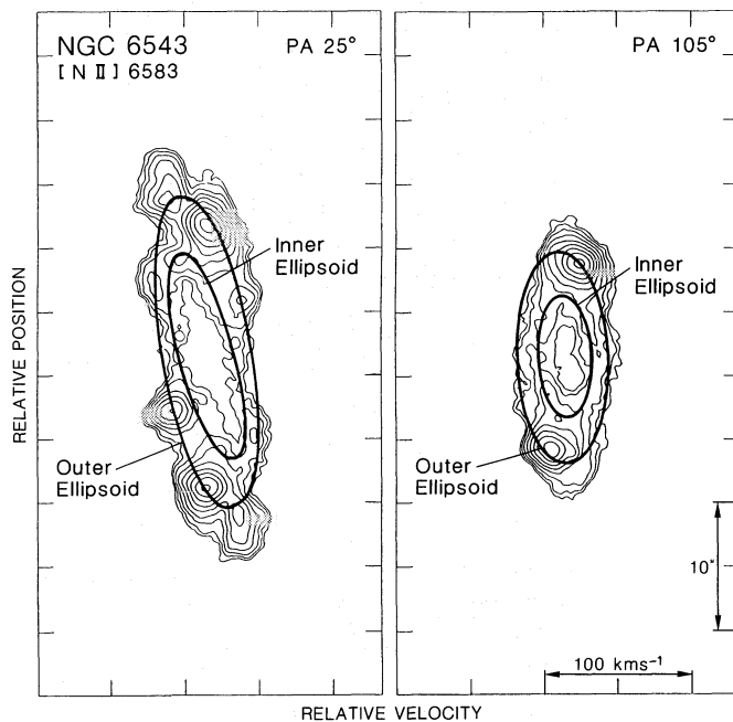
Fig. 8. Elliptical line shapes, at PA 25^\circ and 105^\circ , predicted by the kinematic model using the parameters derived for the Inner and Outer Ellipsoids (Table 4). The schematic line shapes are superimposed on the PV maps of [N II] at the corresponding PAs
