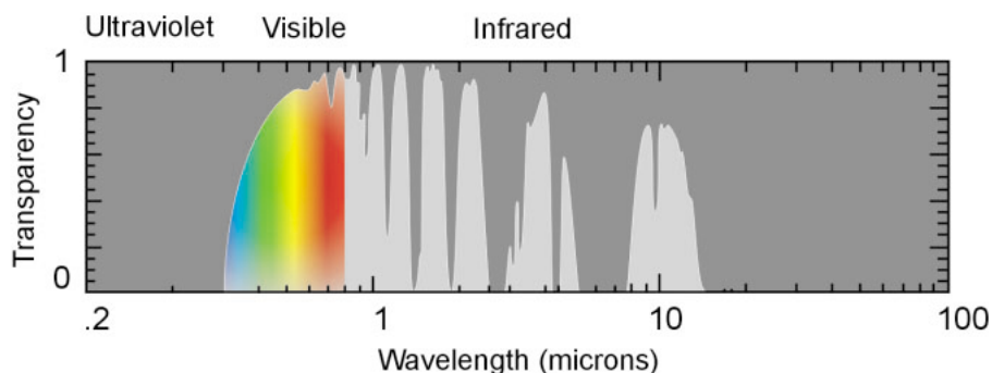
Figure 1: Absorption of radiation by the Earth's atmosphere
