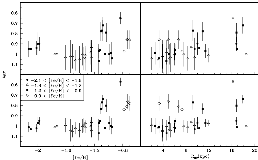
FIG. 5.—Normalized relative ages for our GGC sample from the vertical ( top ) and the horizontal ( bottom ) methods plotted vs. the metallicity ( left ) and vs. Galactocentric distance ( right ). The different symbols represent clusters in different metallicity groups as indicated in the bottom left panel. The error bars are the mean errors as given in cols. (3) and (5) of Table 2. The youngest cluster ( asterisk ) is Pal 12.
