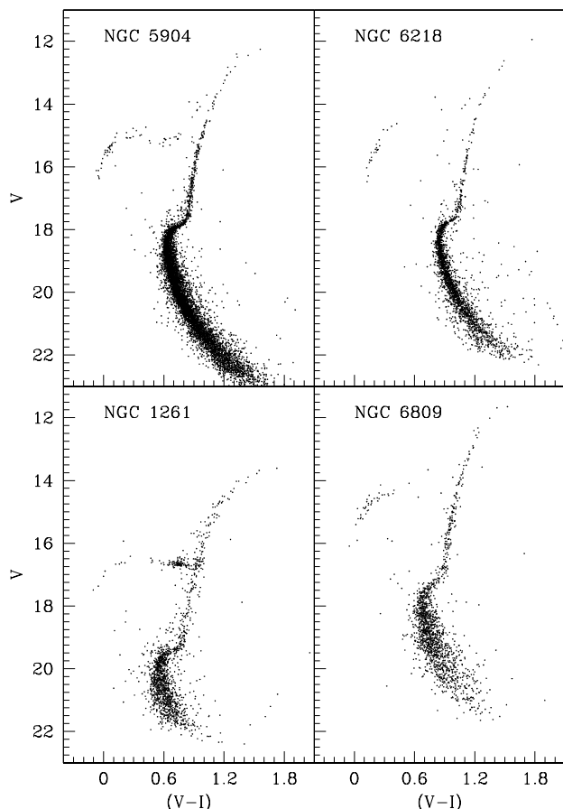
FIG. 1.—CMDs of four clusters used in the relative-age determination, which show the range in quality that is spanned by the present data set. Top , two of the best CMDs (for the clusters NGC 5904 and NGC 6218); bottom , NGC 6809 and NGC 1261 are an example of lower quality photometric samples. In each case, the HB is populated by a good number of stars, and more than 1 mag below the TO is covered even in the case of NGC 1261.
