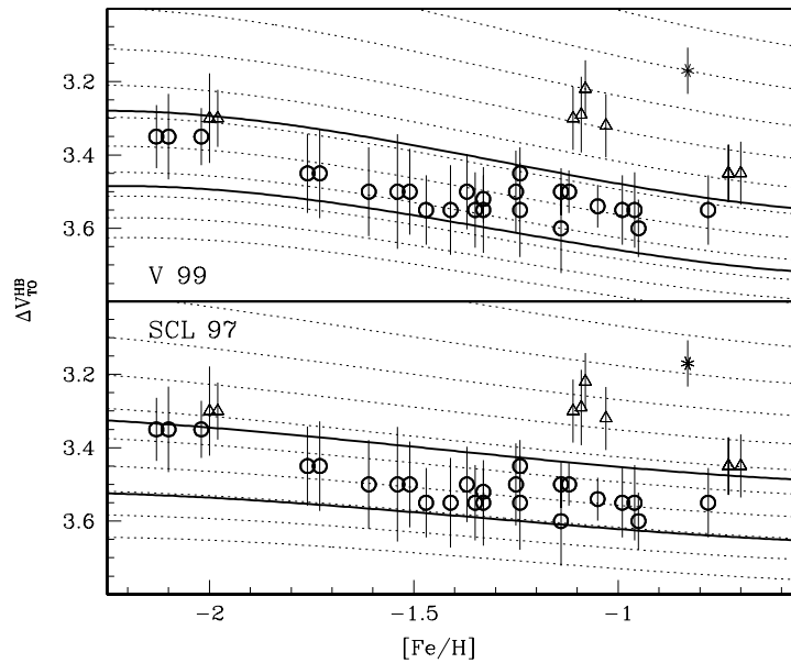
FIG. 3.—Measured \Delta V_{TO}^{HB} parameter plotted vs. the metallicity. The dotted lines in the two panels show the theoretical trend for V99 ( top ) and SCL97 ( bottom ) models. The isochrones are spaced by 1 Gyr (starting from 18 Gyr at the bottom). The asterisk represents the cluster Pal 12. The two isochrones displayed as solid lines represent the \pm 1 standard deviation limits of the \Delta V_{TO}^{HB} parameter for the entire sample (excluding Pal 12), and clusters falling within these ( circles ) are defined as “fiducial coeval” clusters. Note that the two independent models give the same fiducial coeval object selection.
