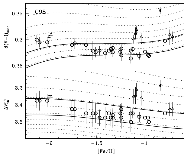
FIG. 9.—Same as Figs. 3 and 4, but for the models of C98
