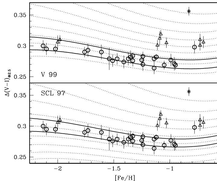
FIG. 4.—Measured \delta(V-I)_{2.5} parameter plotted vs. metallicity. The same two sets of theoretical models of Fig. 3 are shown ( dotted lines ). Age is spaced in 1 Gyr steps, the bottommost line corresponding to 18 and 17 Gyr isochrones, for V99 and SCL97, respectively. The fiducial coeval clusters selected in Fig. 3 are plotted as open circles. The two isochrones displayed as solid lines represent the \pm 1 standard deviation limits of the \delta(V-I)_{2.5} parameter for the GGC sample (except Pal 12). Notice that the two clusters at [Fe/H] = -0.73 (NGC 6366 and NGC 6838) have the same \Delta V_{TO}^{HB} , so they appear as a single point in Fig. 3.
