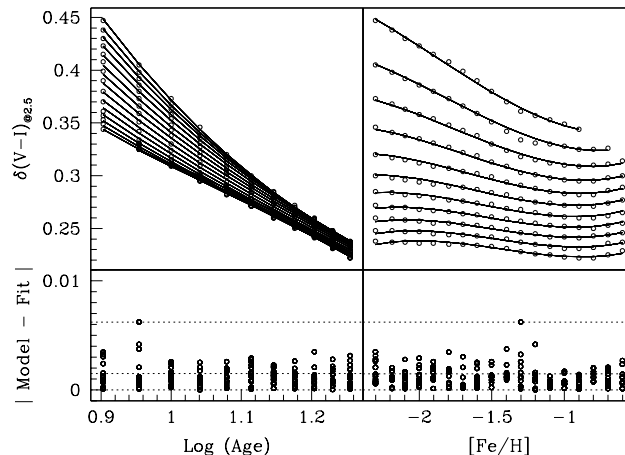
FIG. 8.—Example of our fit to the SCL97 models. The measured values on the theoretical models are fitted in both the \delta(V-I)_{2.5} vs. [\text{Fe}/\text{H}] plane (top right) and the \delta(V-I)_{2.5} vs. \log t plane (top left). The fits to the theoretical values (open circles) are shown as continuous lines. The bottom panels show the residuals.
