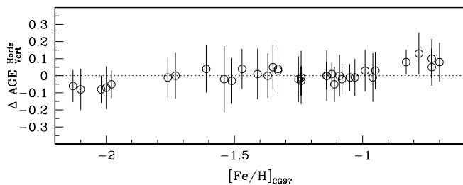
FIG. 6.—Difference in the normalized relative ages obtained from the two methods, \Delta \text{AGE}_{\text{Vert}}^{\text{hor}} , as a function of the metallicity. The error bars were obtained as the quadratic sum of the errors from the two methods.
