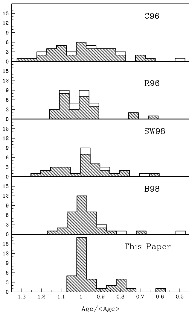
FIG. 7.—Histograms of the relative-age distribution from the most recent compilations in the literature. The histograms are centered on the mean age of the respective samples. Clusters located at the right are younger. The hatched zone represent the clusters within 20 kpc from the center of our Galaxy. The labels identify previous investigations, as explained in the text.
