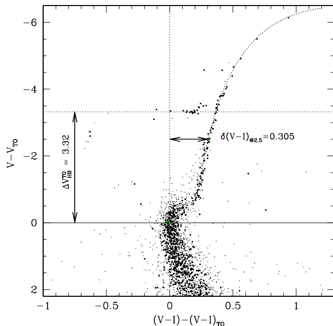
FIG. 2.—CMD of NGC 1851. The heaviest points represent the selected CMD used to measure the TO position and to fit the RGB fiducial line. Magnitude and color have been registered to the TO point. The vertical \Delta V_{\text{TO}}^{\text{HB}} and horizontal \delta(V-I)_{2.5} parameter values for this cluster are indicated by arrows. The analytical fit to the RGB is also shown.
